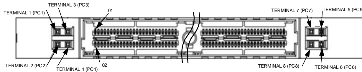
QMS/QFS PC4 terminal ( PC1 .. PC8 ) assignments – front view - 2 bank connector is shown
