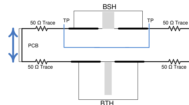
ZX134CS - Simplified Circuit Diagram
