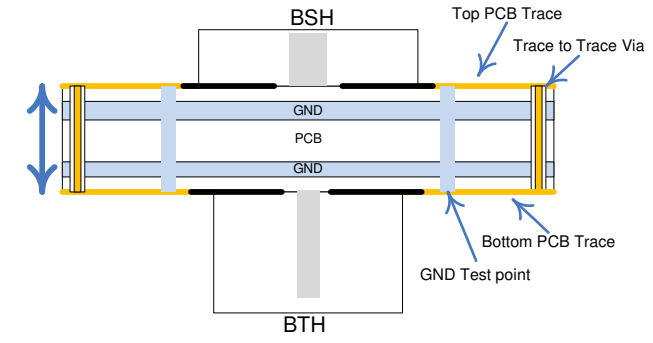
ZX134CS Cross section view
