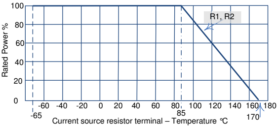
Figure 4 – Current sense resistor Derating chart
