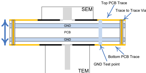
ZX117HS8-CS30 Cross section view
