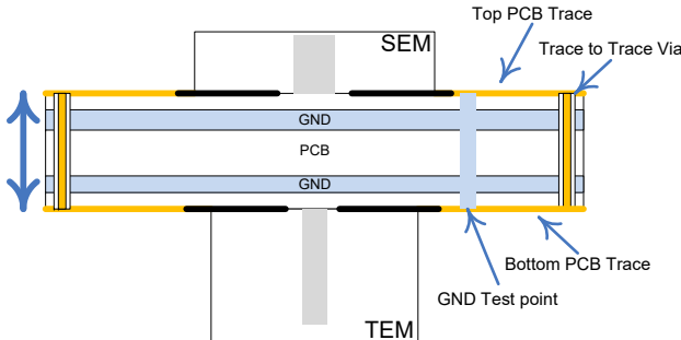
ZX117HS8-CS15 Cross section view
