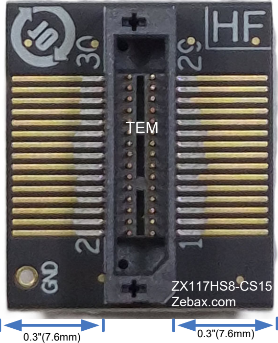
ZX117HS8-CS15 Bottom View
