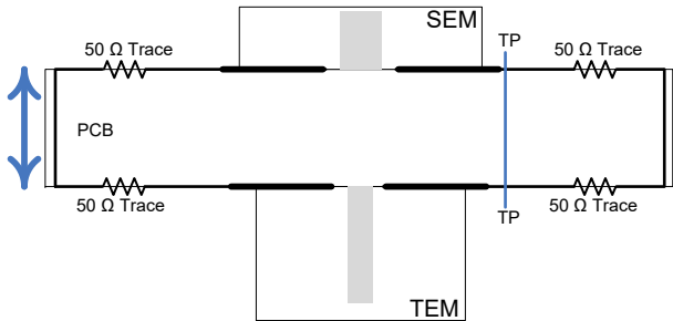
ZX117HS8-CS15- Simplified Circuit Diagram
